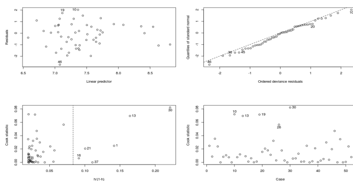
Figure B.4: Diagnostic plots for 4-grams
