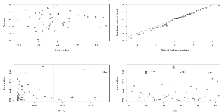
Figure B.3: Diagnostic plots for 3-grams
