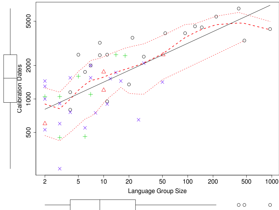
Figure 10.1: Calibration dates against the number of languages in a language group. os are archaeological, △s are archaeological and historical, +s are epigraphic and xs are historical dates.
