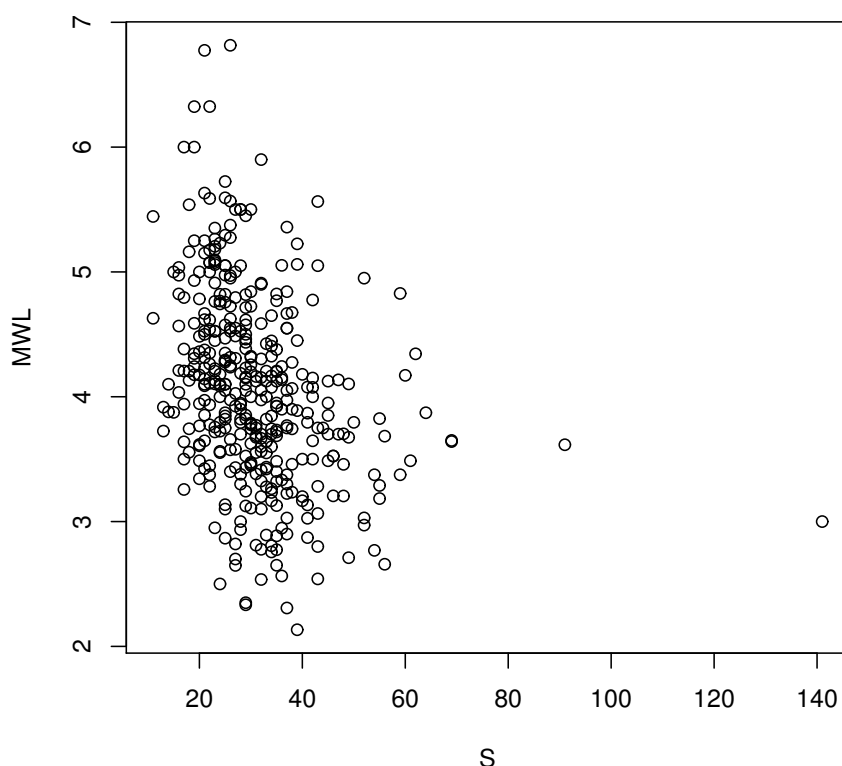
Figure 7.2: Mean word length from ASJP data plotted against segment inventory sizes from UPSID
