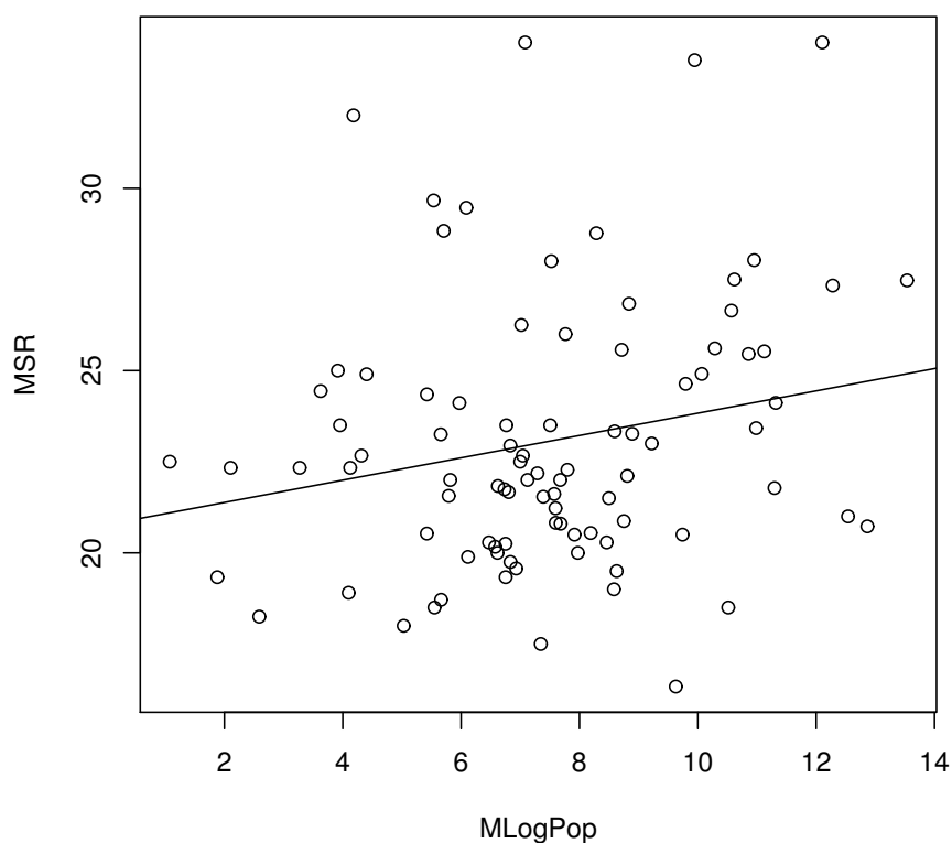
Figure 7.8: Mean of segments represented in ASJP word lists within families with 2 or more speakers plotted against the mean of log of population sizes
