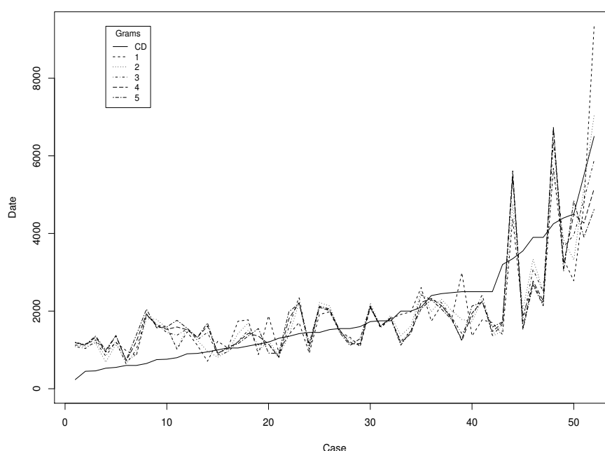
Figure 10.3: Comparing predicted dates for various n-grams
