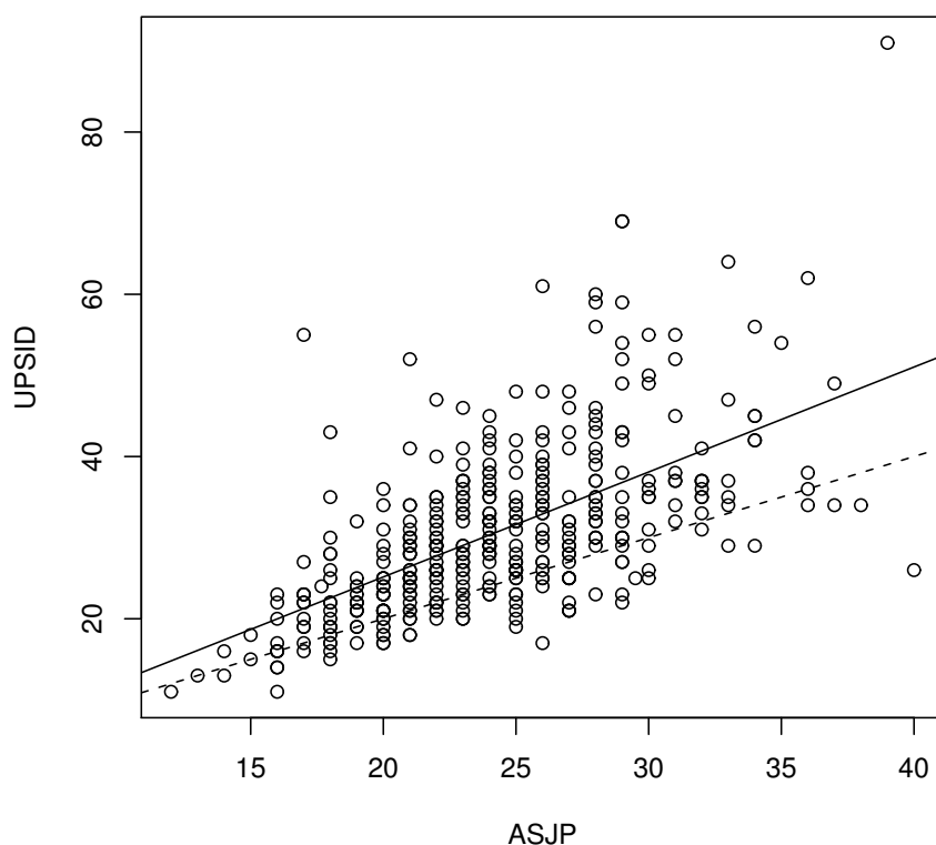
Figure 7.1: Numbers of segments in languages that are in both ASJP and UPSID. The solid line is based on a linear model predicting UPSID segment inventory size from the number of segments (SR) in ASJP word lists. The dotted line, with an intercept at (0, 0) and slope of 1, separates cases with respectively more (above the line) or fewer (below the line) UPSID segments than SRs
