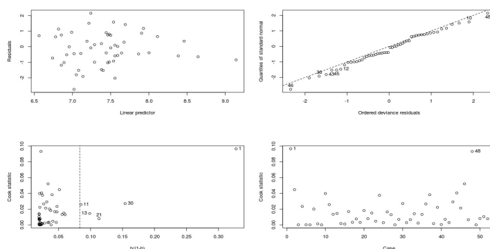
Figure B.1: Diagnostic plots for 1-grams
