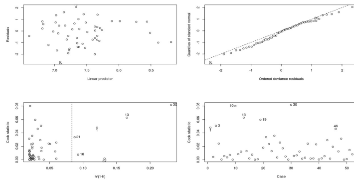
Figure B.5: Diagnostic plots for 5-grams
