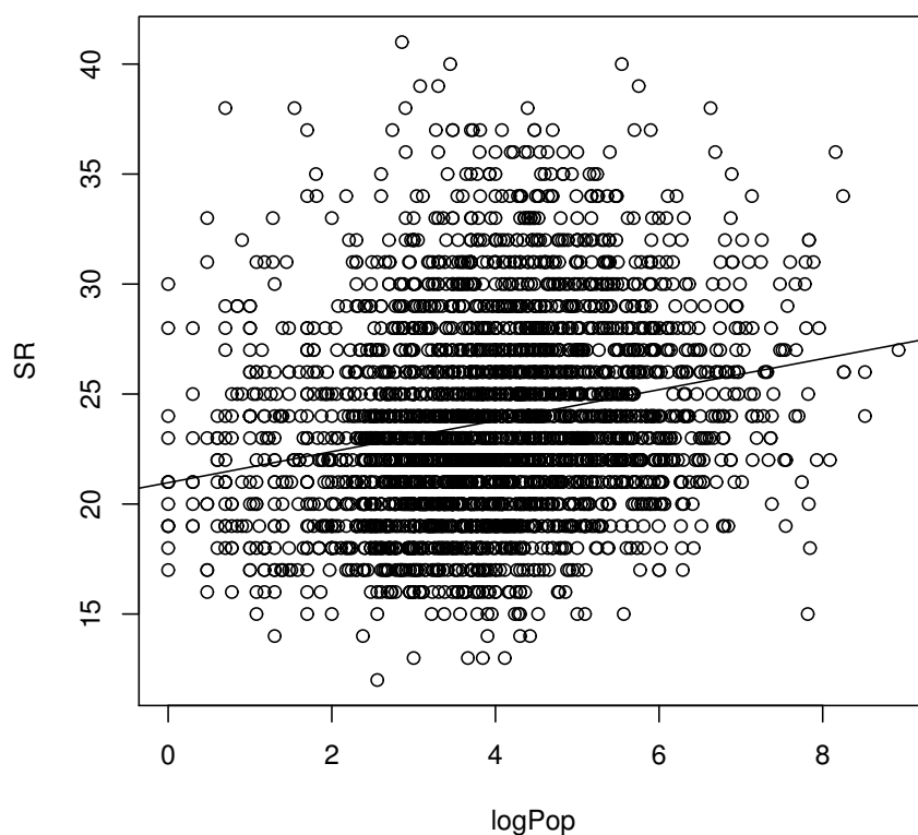
Figure 7.7: Segments represented in ASJP word lists for individual languages with one or more speakers plotted against log of population sizes from Lewis 2009
