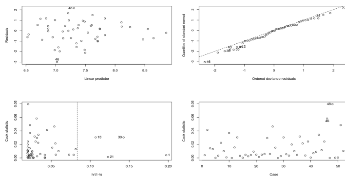
Figure B.2: Diagnostic plots for 2-grams
